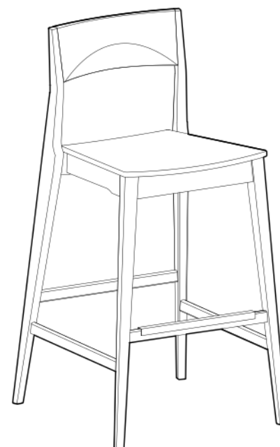
LH-42 ply seat barstool • W 541mm (21 5 / 16 "") D 578mm (22 3 / 4 "") H 1075mm (42 5 / 16 "")
