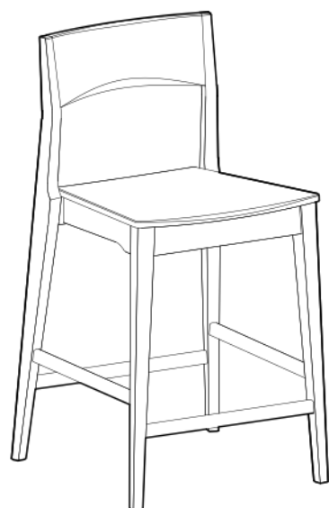
LH-42 ply seat counterstool • W 518mm (20 6 / 16 "") D 547mm (21 1 / 2 "") H 947mm (37 4 / 16 "")
